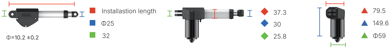
Speed and force (2600rpm)
